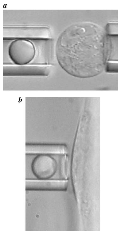
FIGURE 1 The microscopic view of single tether extraction from suspended or attached HUVECs with the micropipette-aspiration technique. ( a ) The experimental setup for extracting single tethers from a suspended HUVEC, which was held with a micropipette as shown. The bead, which fits snugly in the micropipette, acts as the force transducer. ( b ) The experimental setup for extracting single tethers from a surface-attached HUVEC, which was cultured on the side wall of the experimental chamber.
